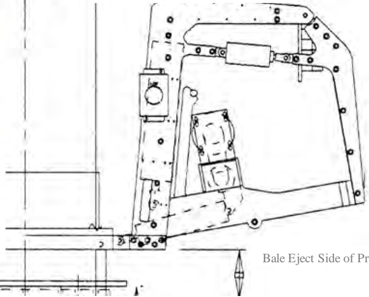
Model P600 Bale Tying System on Press with Doors
