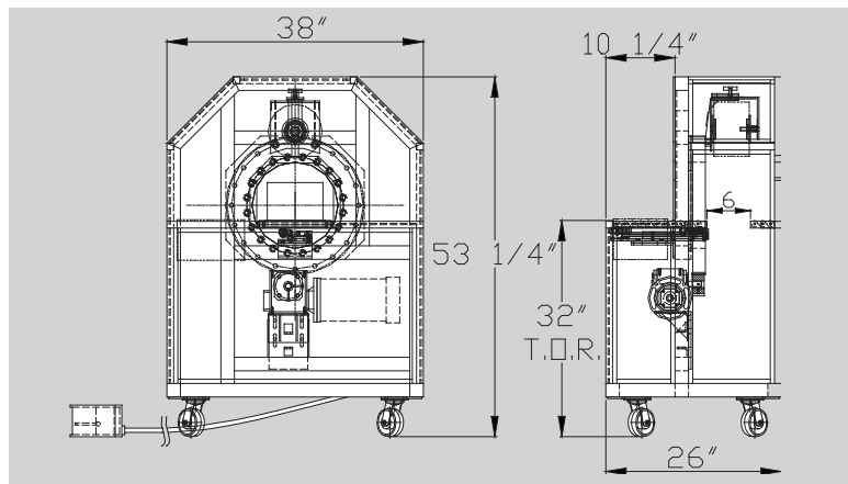
Bander with 12.75" Ring I.D diameter and 1 HP Drive
